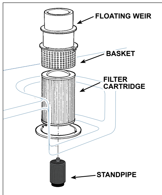
FILTER SYSTEM
